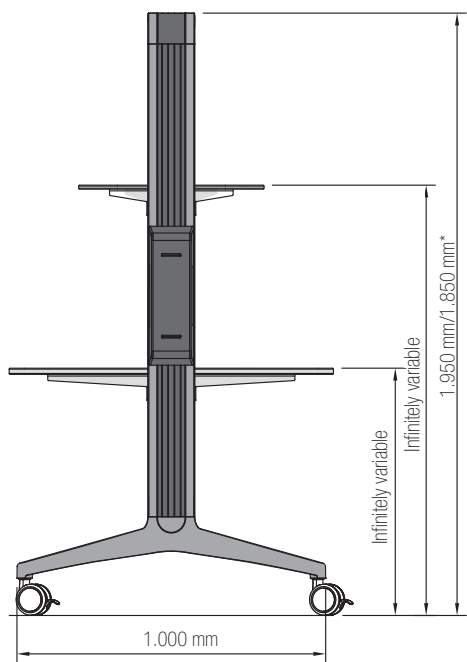
Type T 1050 * Height for stationary type with swivel base plate
