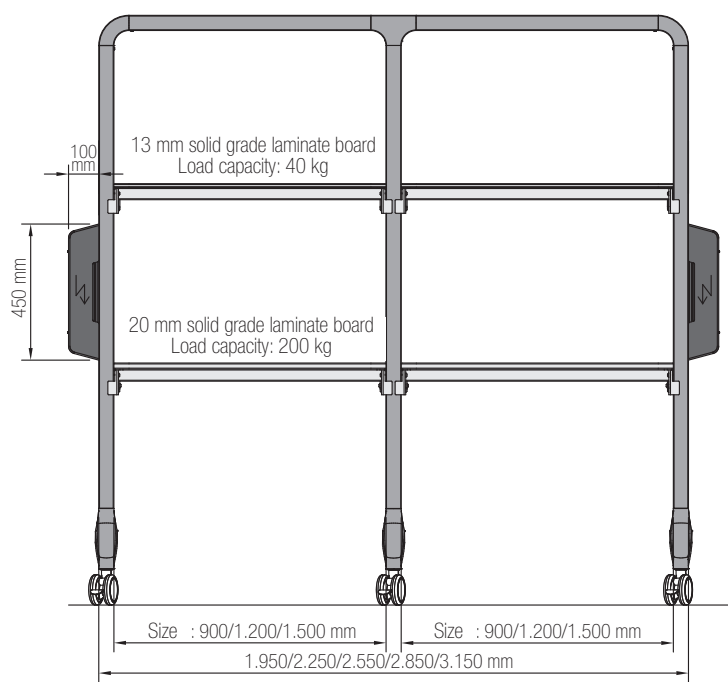
Type T 800 | Mobile basic module and add-on module Total load capacity: 450 kg
