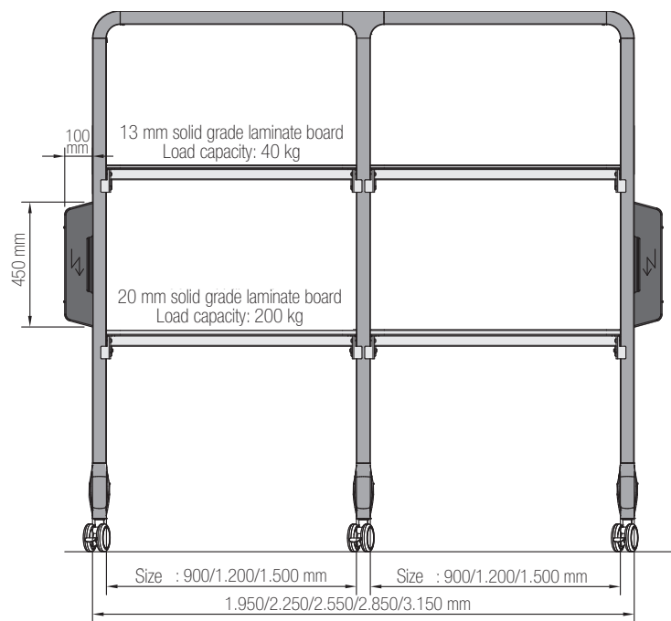
Type T 1050 | Mobile basic module and Add-on module Total load capacity: 450 kg
