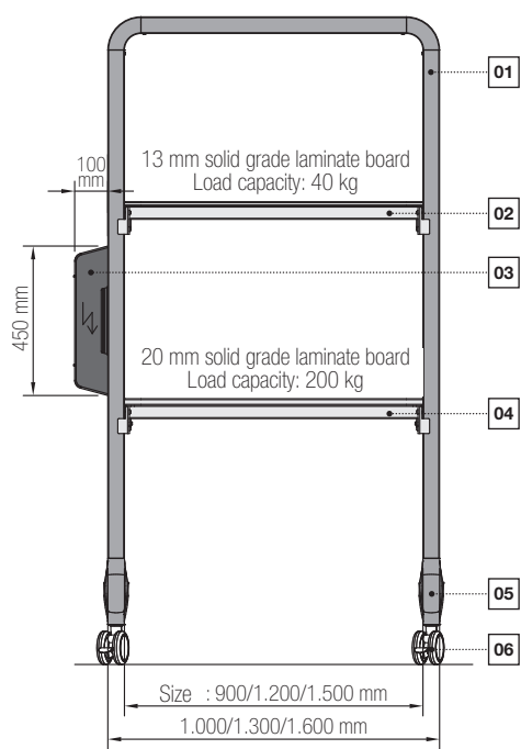
Type T 800 | Mobile single module Total load capacity: 300 kg
