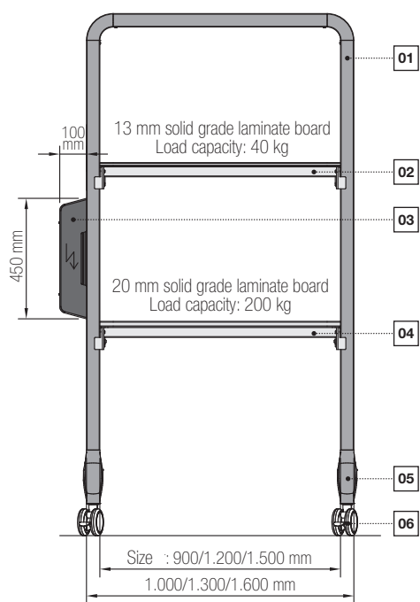
Type T 1050 | Mobile single module Total load capacity: 300 kg
